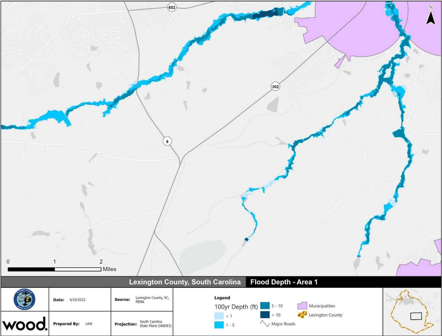
FIGURE 6.32 – LEXINGTON COUNTY FLOOD DEPTH GRID (100-YR) – AREA 1
